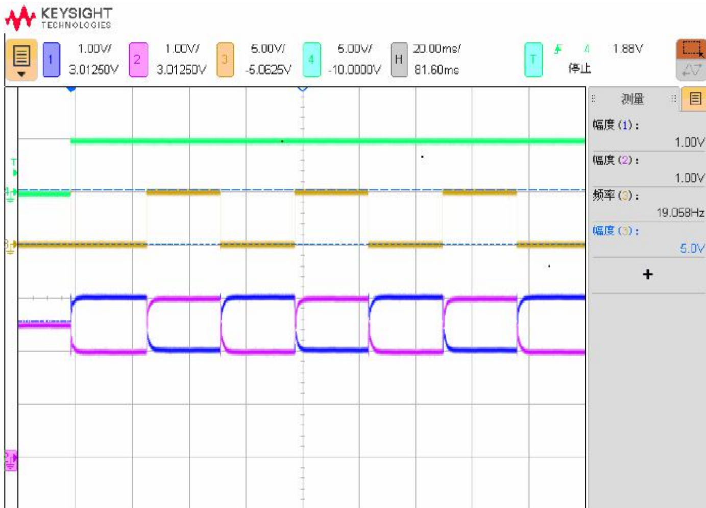
Channel 1: OUTP, Channel 2: OUTN, Channel 3: STDO, Channel 4: STEN
